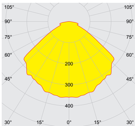
cd/klm — C0 - C180
