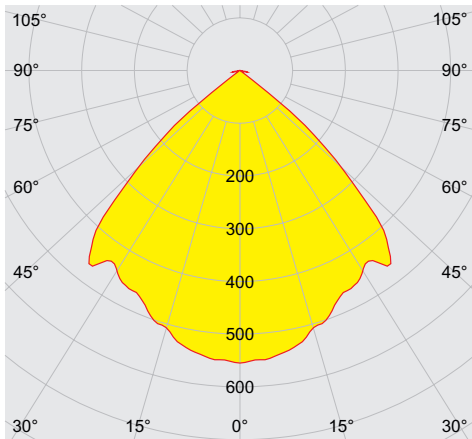
cd/klm \eta = 100\% — C0 - C180
