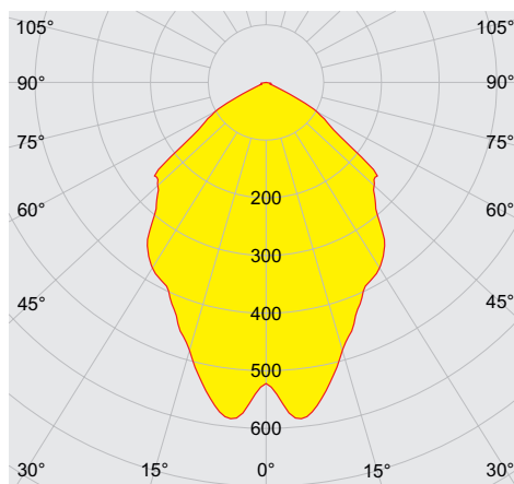
cd/klm — C0 - C180
